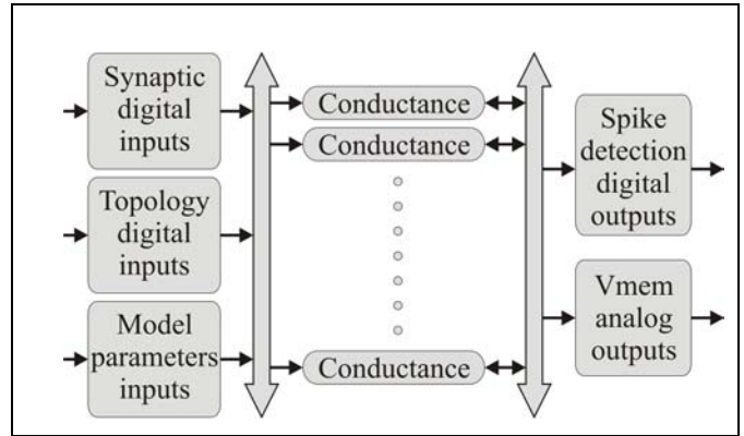
Fig. 2 : Galway chip architecture and data I/O
